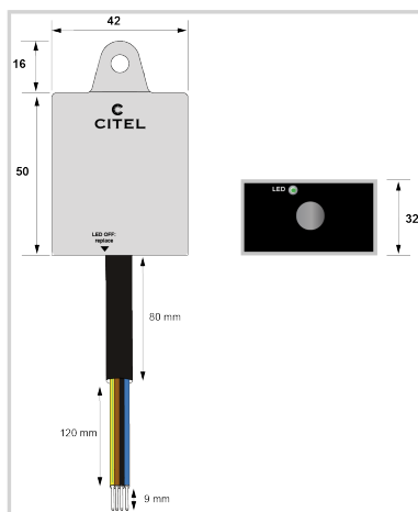
MLPCA1-230L-2L
