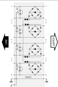
G: 3-electrode gas tube
