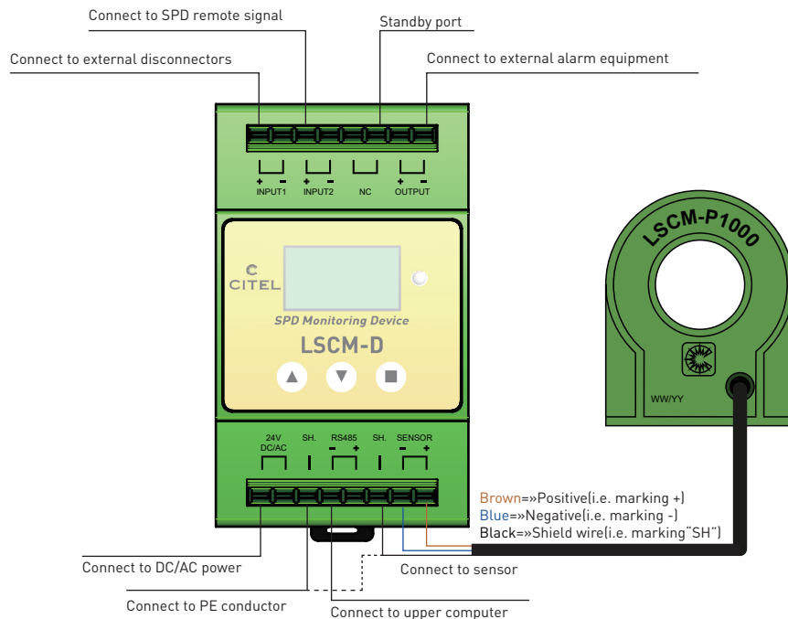
Fig3. Typical LSCM-D wiring connection
