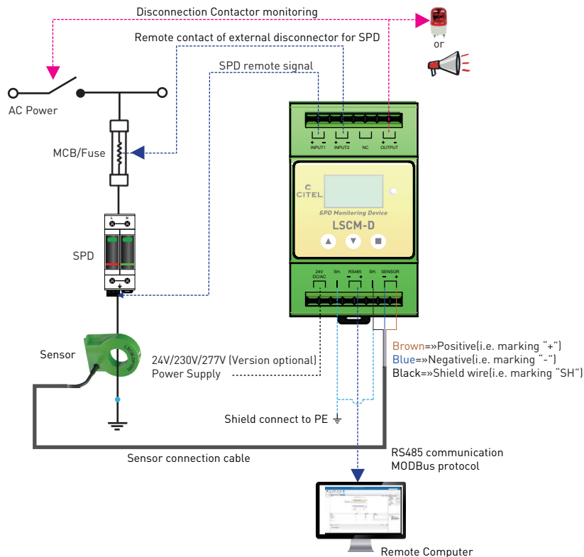
Fig4. Typical wiring diagram for LSCM-D
