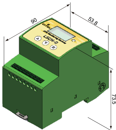
Monitoring unit LSCM-D
