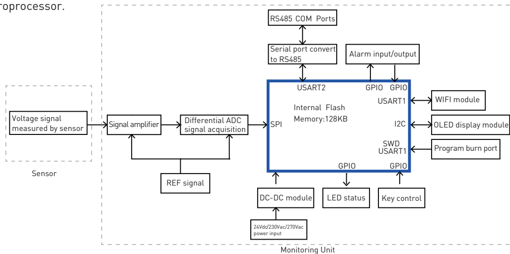
Fig1. LSCM-D system schematic diagram
